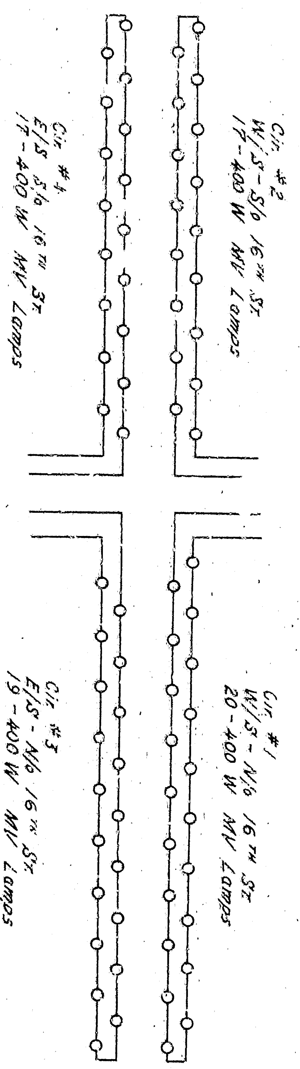
CIRCUIT DIAGRAM No Scale
