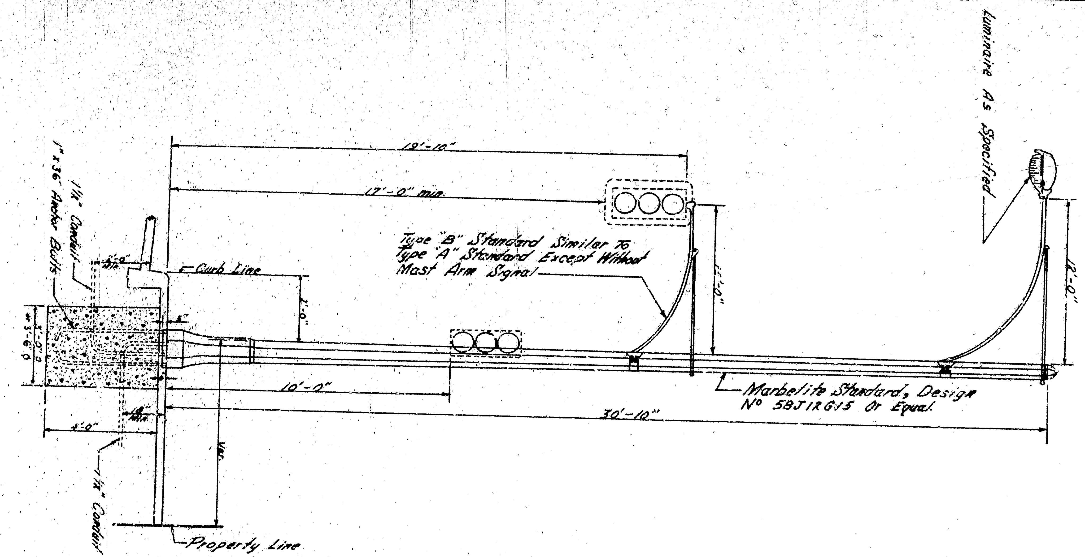
TYPE III (a) STANDARD as shown
