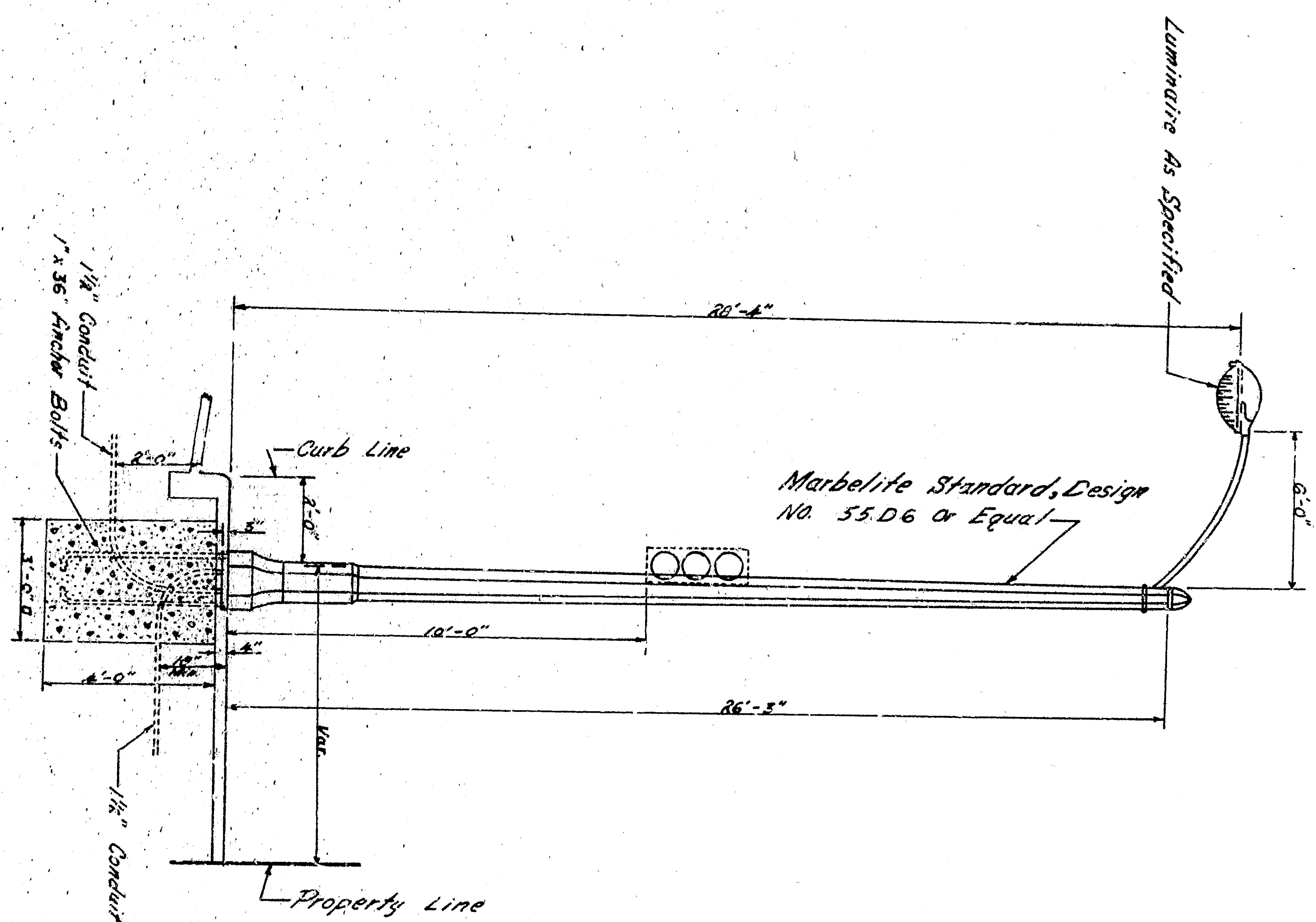
TYPE X (a) STANDARD, as shown (Signal inserts only)
